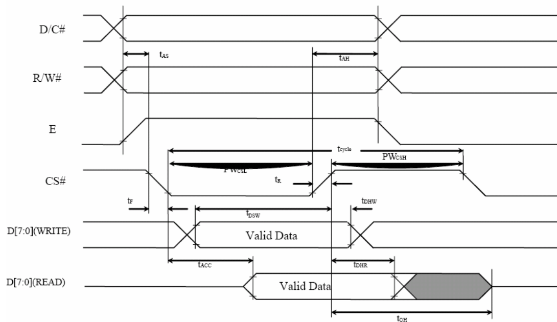
Figure 13-3 : 6800-series MCU parallel interface characteristics
